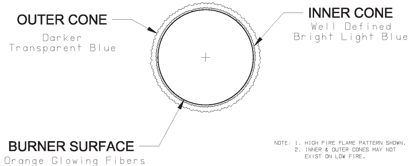
Figure 3: Burner Flame
